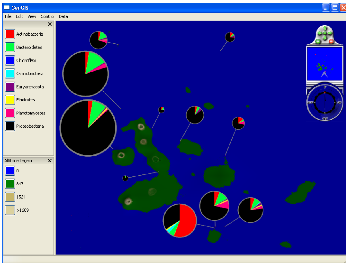
Figure 1: phylum association of proteorhodopsin-like sequences collected from eleven sample sites in the Galapagos Islands archipelago. The main frame contains the OpenGL canvas and displays digital elevation data, pie charts showing the total count (size) and relative proportion (wedge size) of proteorhodopsin sequences, and control elements including the minimap. Classification and elevation legends are shown in the left-hand panels.
